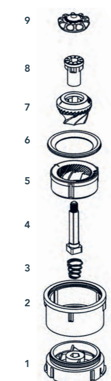
1. Base 2. Housing 3. Spring 4. Shaft 5. Crown 6. Bottom Ring 7. Cone 8. Cone holder 9. Adjusting wheel
